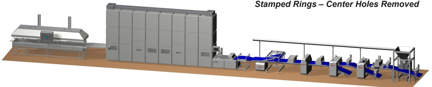
Yeast Raised Donut System with Stamper
