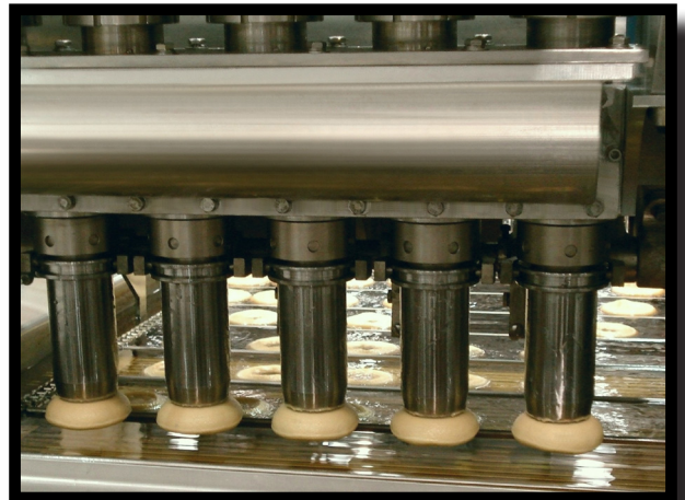
Fill-O-Matic Depositor in Operation
