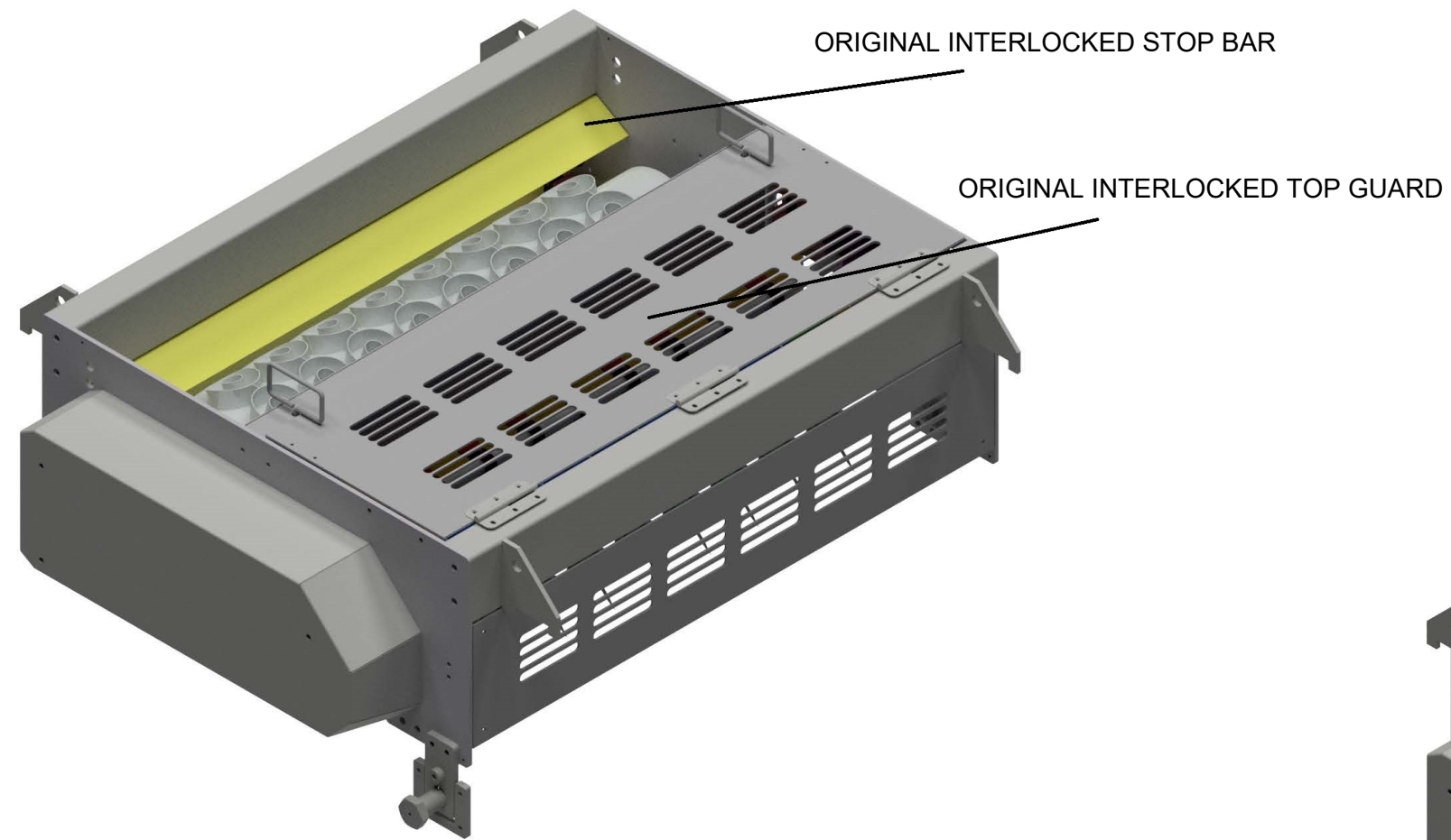
MOLINE CUTTER/PICKER UNIT WITH ORIGINAL INTERLOCKED TOP GUARD AND STOP BAR
