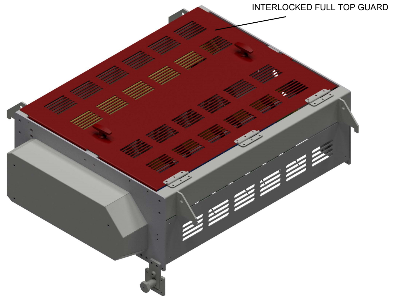
MOLINE CUTTER/PICKER UNIT WITH REDESIGNED INTERLOCKED FULL TOP GUARD
