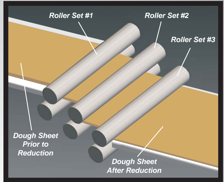
Dough Travel Through Rollers
