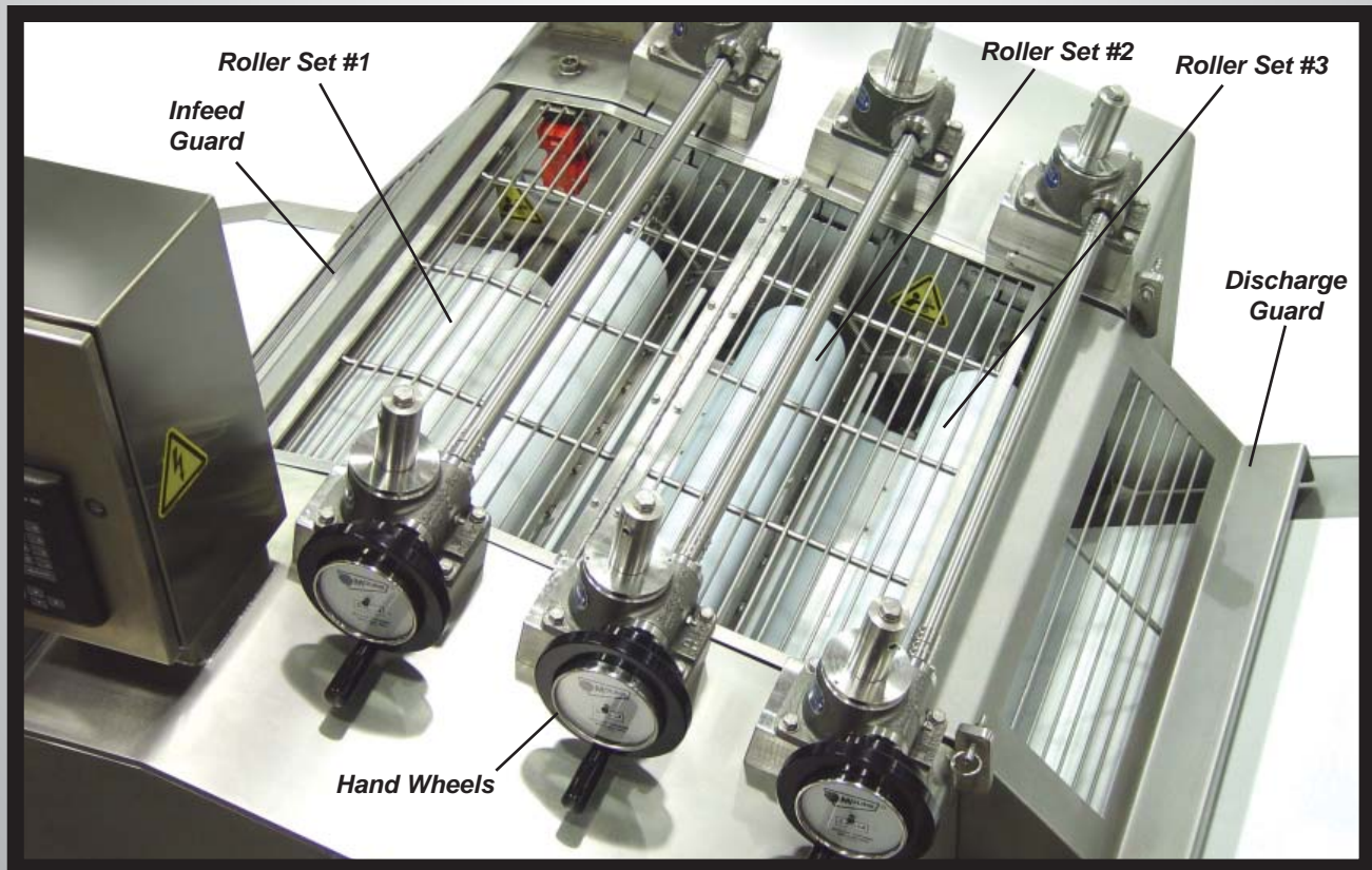
Dough Reduction Unit (top view)
