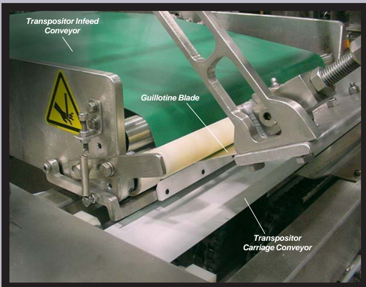
Transpositor Guillotine (on the cutting module)
