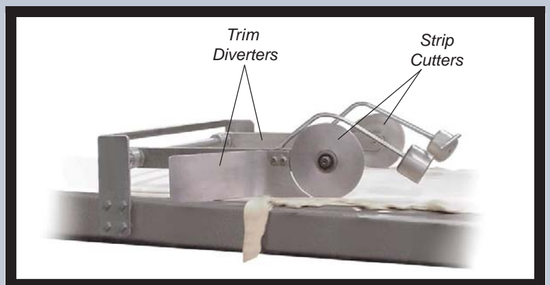
Trim Diverters With Strip Cutter
