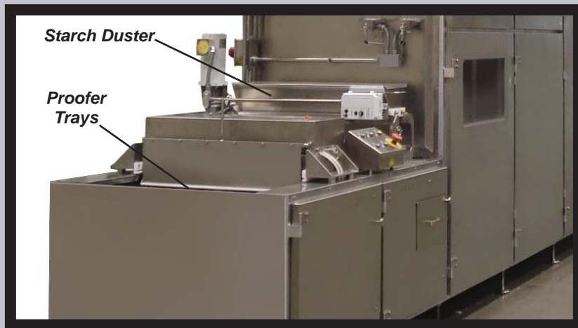
Starch Duster Mounted on a Proofer
