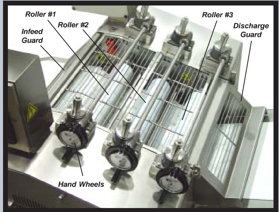
Dough Reduction Unit (top view)
